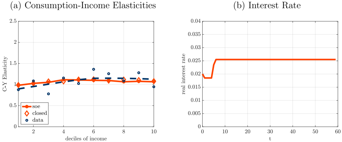
Figure D.9: Consumption and Interest Rate Responses in a Closed Economy
